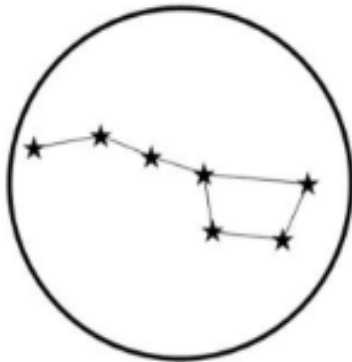
Ursa Major: Great Bear (the Big Dipper)
